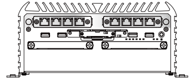
RCO-6011E-8L RCO-6011E-8P
