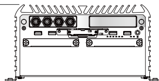
RCO-6022PE-4L-M12 RCO-6022PE-4P-M12
