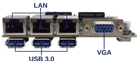
2I610DW Rear I/O
