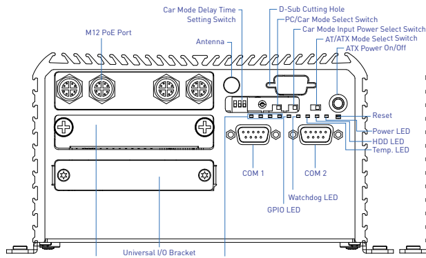
Front Panel
