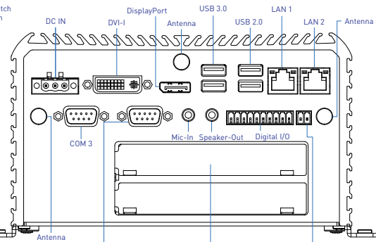
Rear Panel
