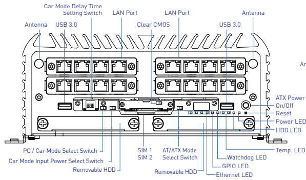
Front Panel
