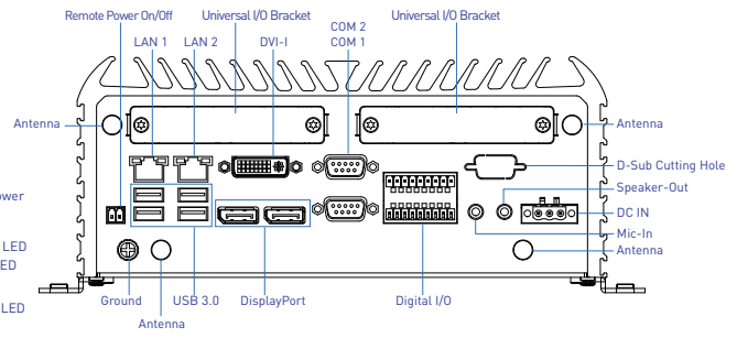
Rear Panel
