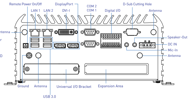
Rear Panel
