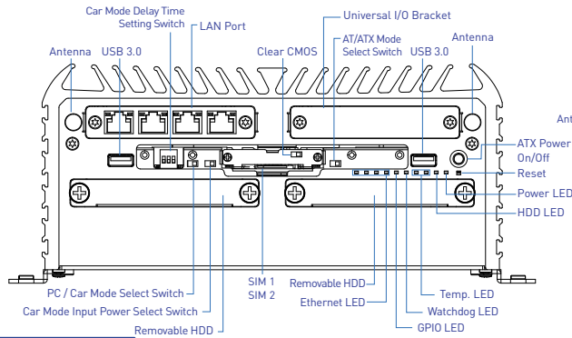
Front Panel
