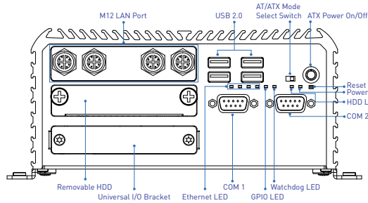
Front Panel
