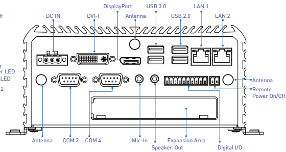
Rear Panel
