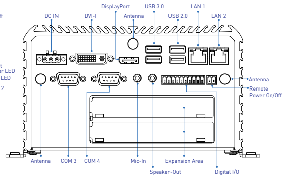
Rear Panel
