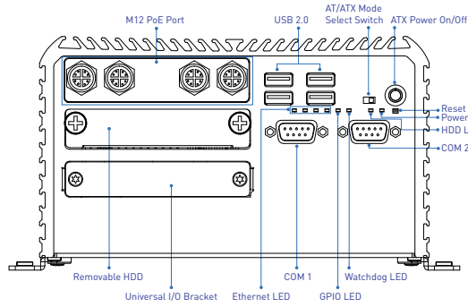
Front Panel
